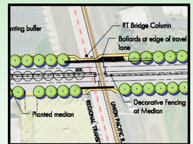
Draft Streetscape Master Plan Section
